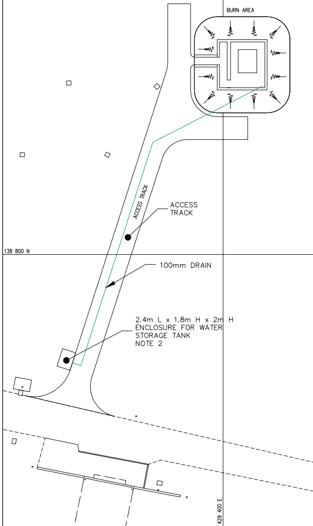
DETAIL (1:500)
